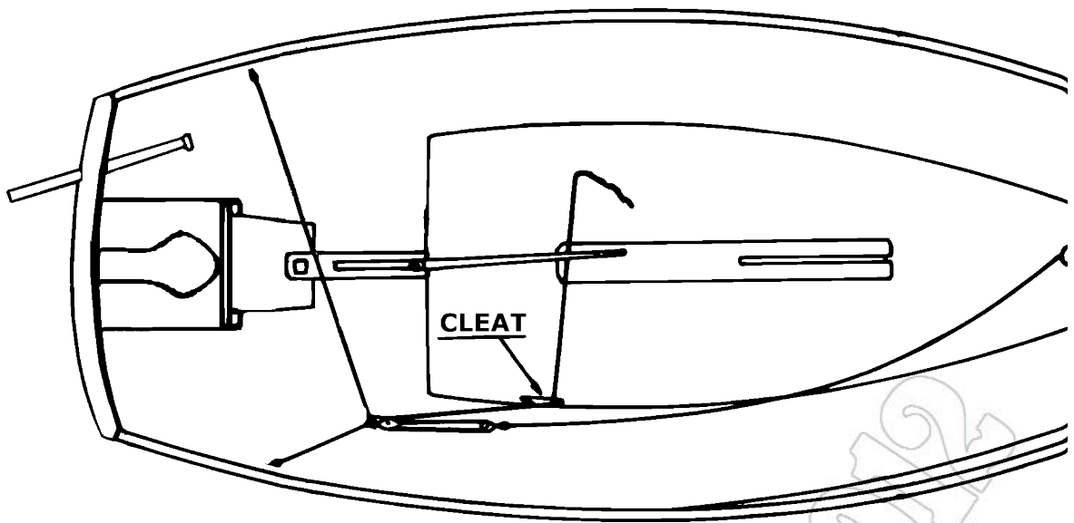
FIG. 4 MAIN SHEET LEAD
